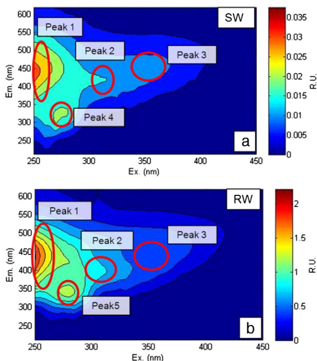
Fig. 5. Average of three replicates Excitation–emission matrices (EEMs) of SW (a) and RW (b). Note the marked difference in the color scale. R.U.: Raman Units.
